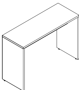
Bancada Alta VBA1263 - 1200x600x1100 VBA1463 - 1400x600x1100 VBA1663 - 1600x600x1100 VBA1863 - 1800x600x1100 VBA2063 - 2000x600x1100
